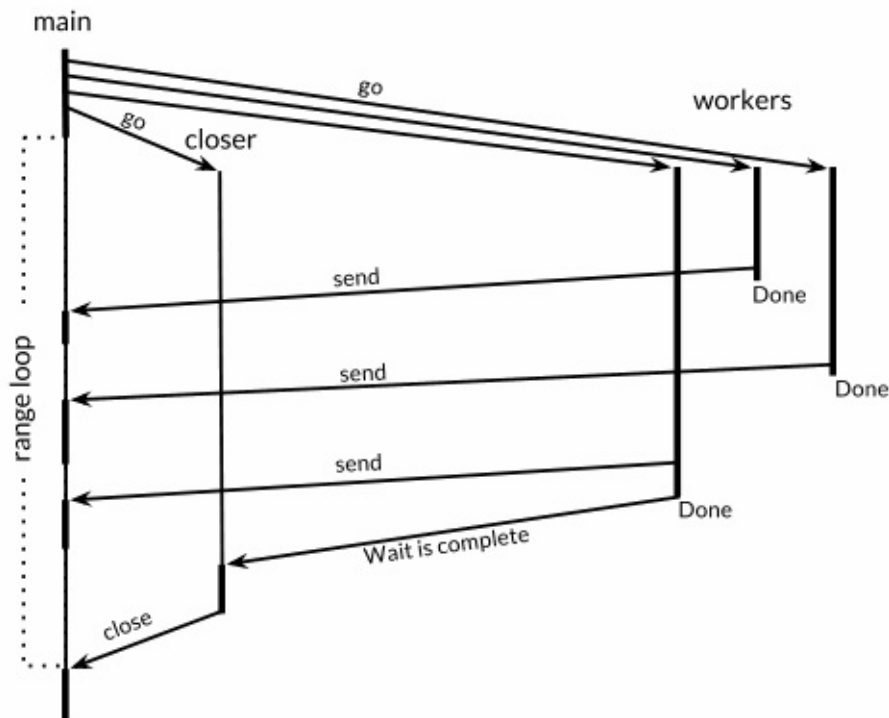
Figure 8.5. The sequence of events in makeThumbnail6 .
